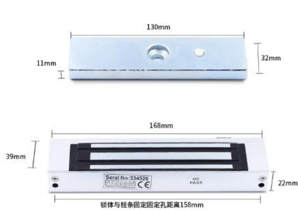
EDL180 Electric magnetic lock
